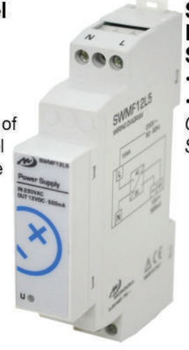
Switching Power Supply • In 230VAC • Out 12V 0.5A Cat No: SWMF12L5
